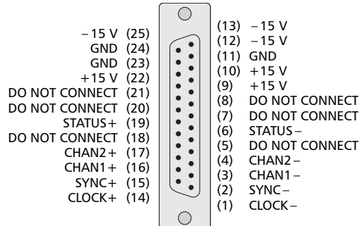
DIGITAL POWER IN (25-pin female D-SUB connector)
